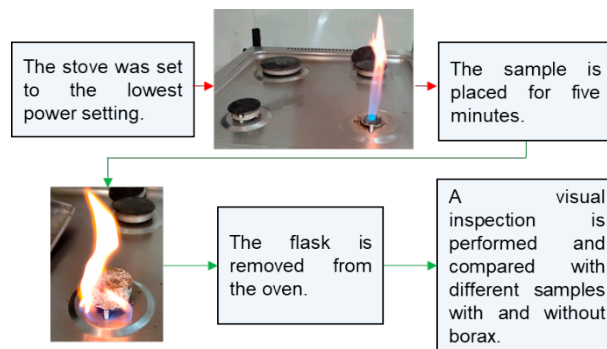
Figure 1. Methodology to be followed to perform the flammability test.
