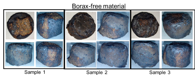
Figure 3. Results in the specimens of the composite material without borax.
