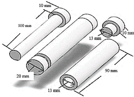
Figure 1. Powder compaction die parts: lower punch, upper punch, die chamber, and die assembly.
