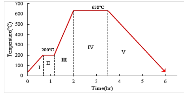
Figure 2. The sintering process.
