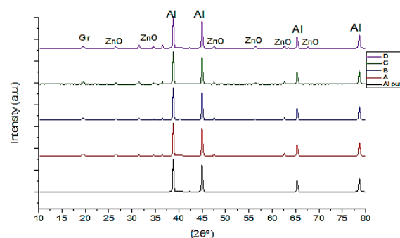
Figure 7. XRD for pure Al and Al + ZnO + Gr.
