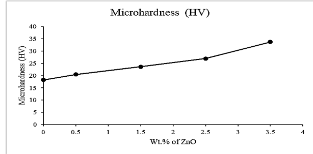
Figure 4. Microhardness values of hybrid nanocomposites
