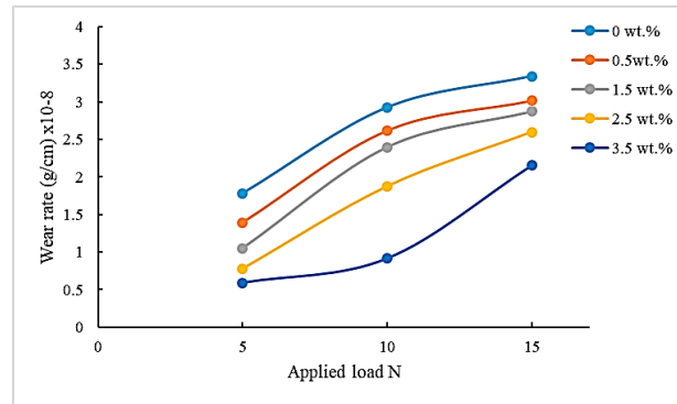
Figure 5. Al/ZnO + Gr wear rate relationship with applied loads.
