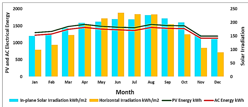
Figure 5. Solar irradiation, DC and AC energy production.
