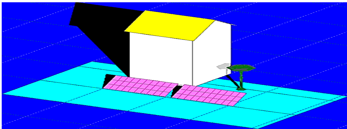
Figure 4. 10 kWp PV solar system design simulation.
