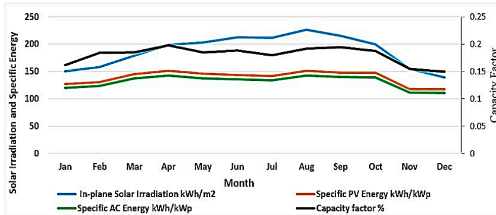
Figure 10: CF, specific PV energy and specific AC energy.
