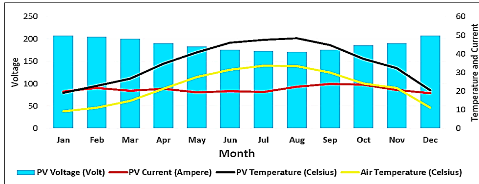
Figure 6. Temperature, voltage, and current.
