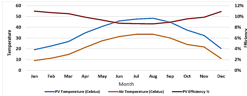
Figure 8. Temperatures and PV module efficiency.
