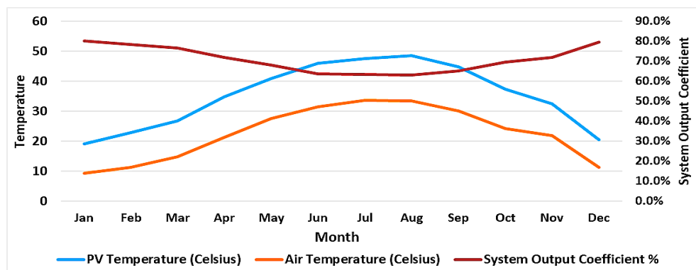
Figure 9. Temperatures, system output coefficient.
