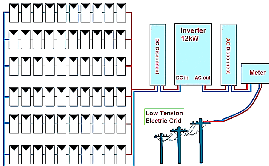
Figure 2. PV solar system single-line diagram.
