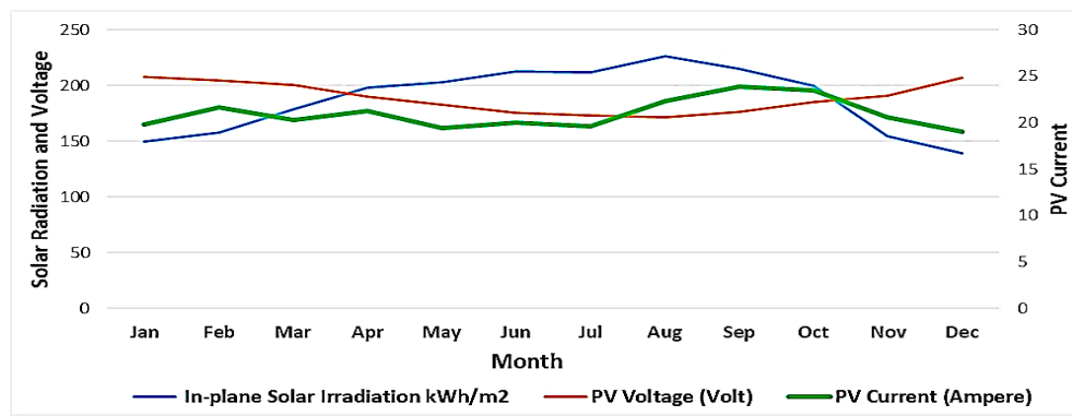
Figure 7. In-plane solar irradiation, voltage, and current.
