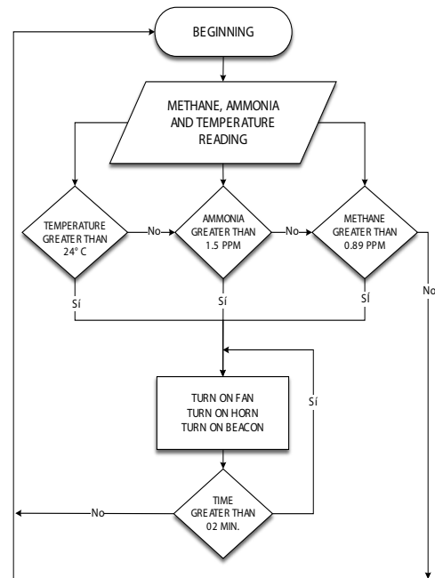
Figure 5. Flow chart of the operation of the control device.
