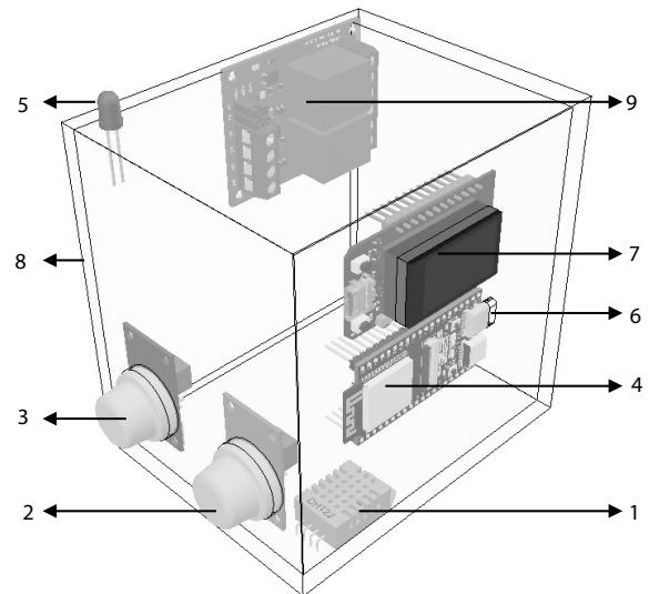
Figure 6. Controller device elements.
