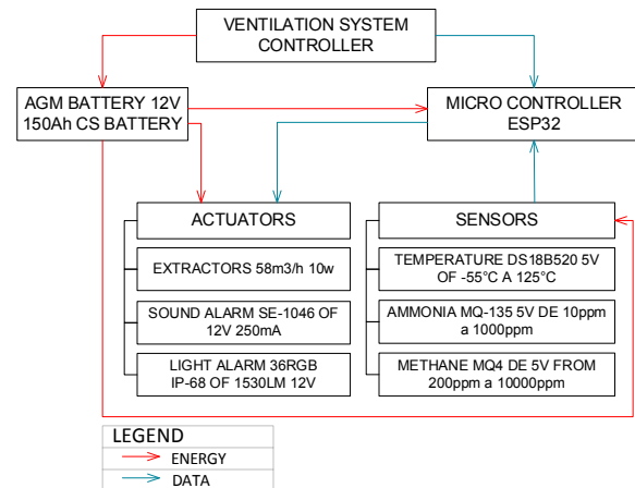
Figure 1. Schematic diagram of the electrical system and instrumentation of the control device.
