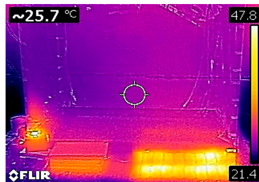
Figure 3. Taking measurements with a Flir C2 thermal imaging camera.
