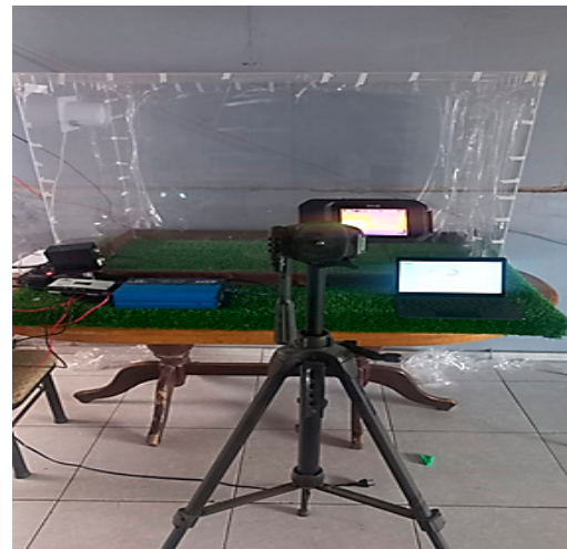
Figure 2. Encapsulation to generate a controlled environment.
