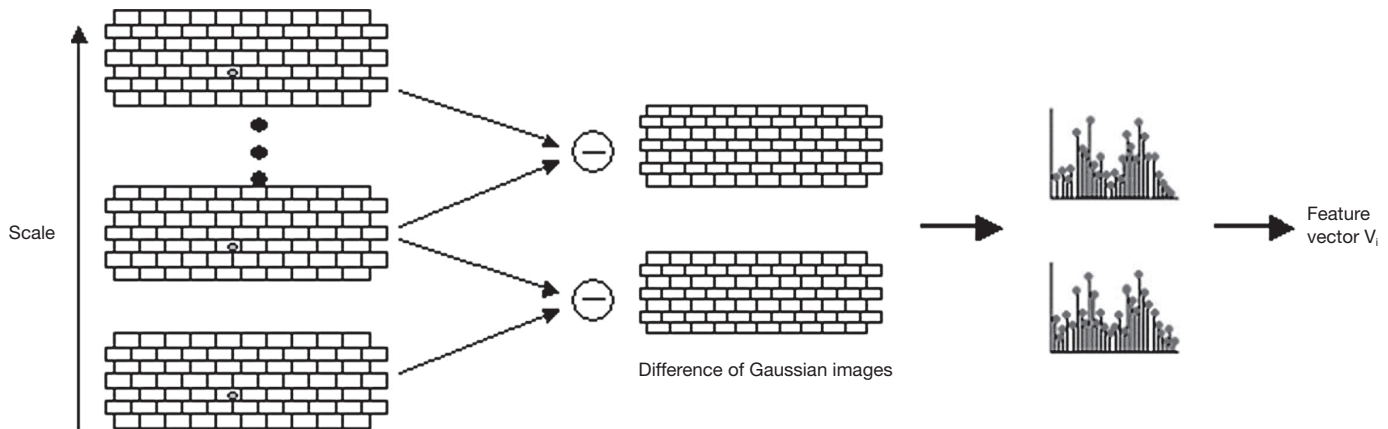
Fig. 2. Snapshot of different scale and it's corresponding DOG image and resultant peak detection using histogram approach.
