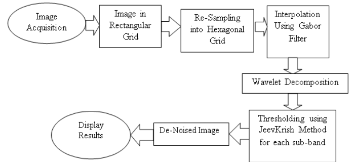
Fig. 5. Block Diagram for the Proposed Method.
