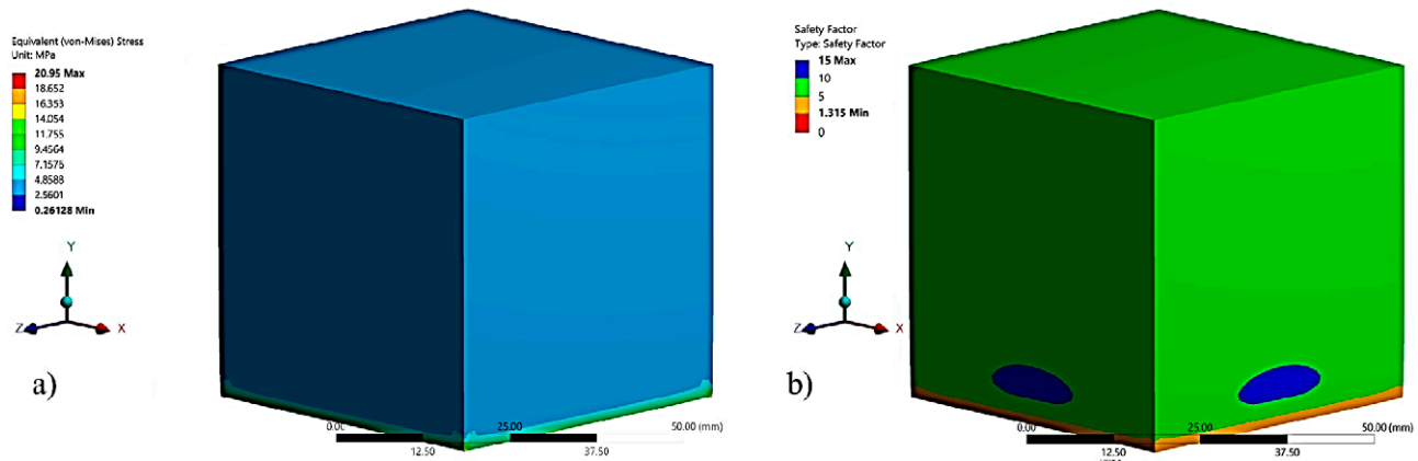
Figure 6. Compression FEA results. a) Equivalent stress and b) safety factor (maximum equivalent stress).
