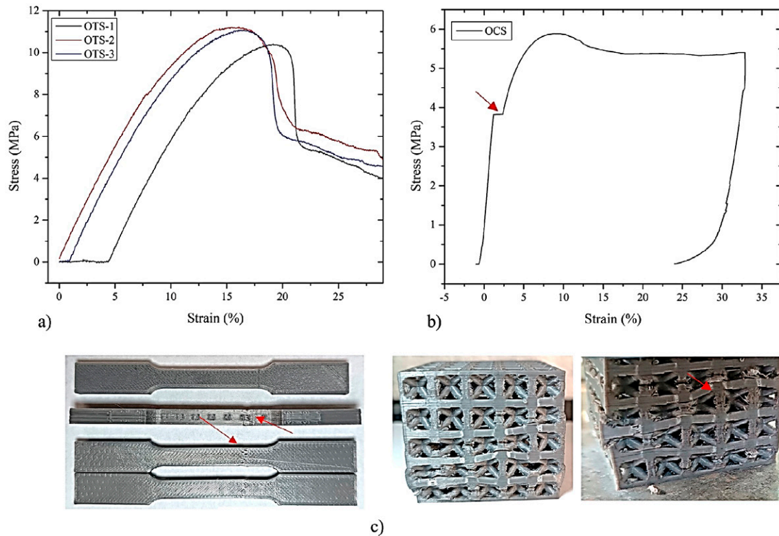
Figure 12. Stress-strain curves. a) Optimized tensile specimens, b) optimized compression specimens, and c) deformations and fractures observed in the tensile and compression specimens evaluated. Some deformed areas are indicated with red arrows.
