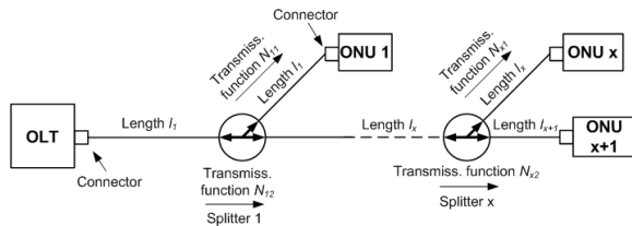
Figure 2. Designed passive optical network with a bus topology.
