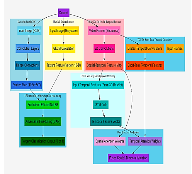
Figure 1. Model Architecture of the Proposed Analysis Process.
