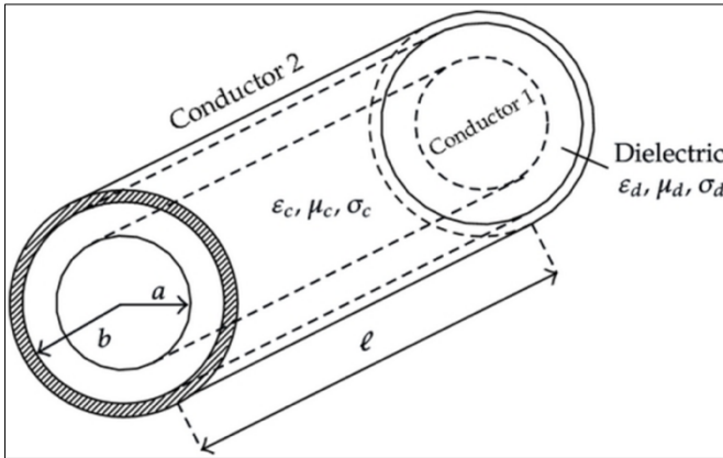
Figure 1: Coaxial line.
