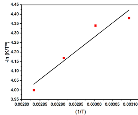
Figure 5. Plot of collision theory for cadmium cementation; m=0.5 ; the initial cadmium concentration of 500 mg/ml.
