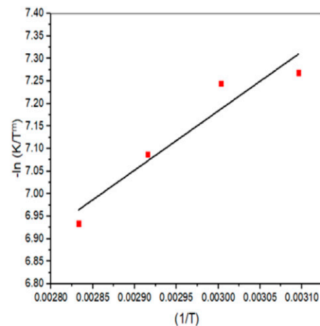
Figure 6. Plot of Transition State theory for cadmium cementation; m=1 ; the initial cadmium concentration of 500 mg/ml.
