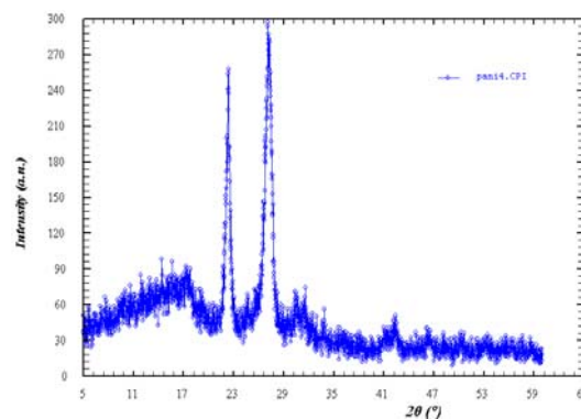
Figure 4. XRD pattern of electrospun polyethylene/polyaniline.
