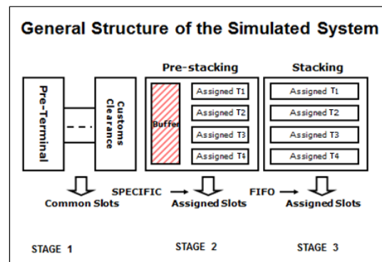
Figure 10. General Structure of the Simulated System.
