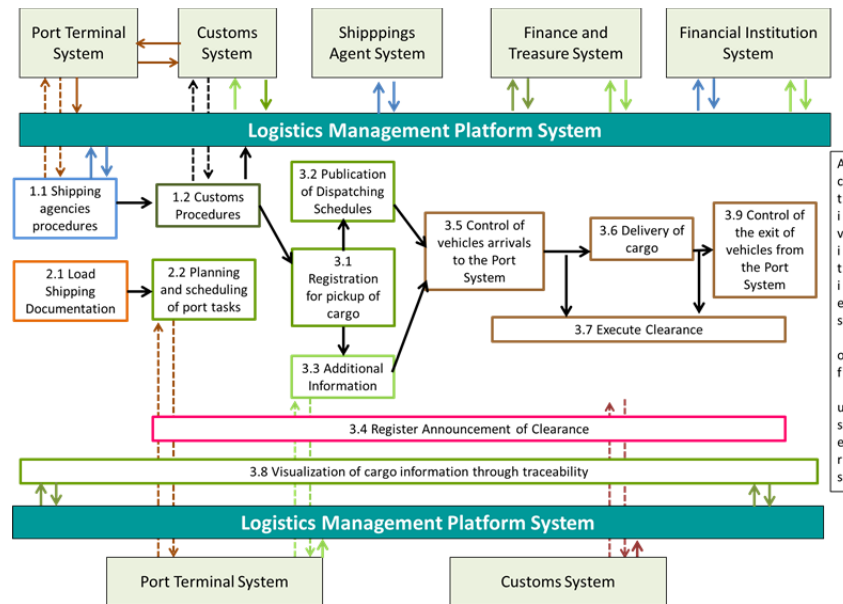
Figure 9. Orchestration of the direct dispatching of import containers flows within the OMS.
