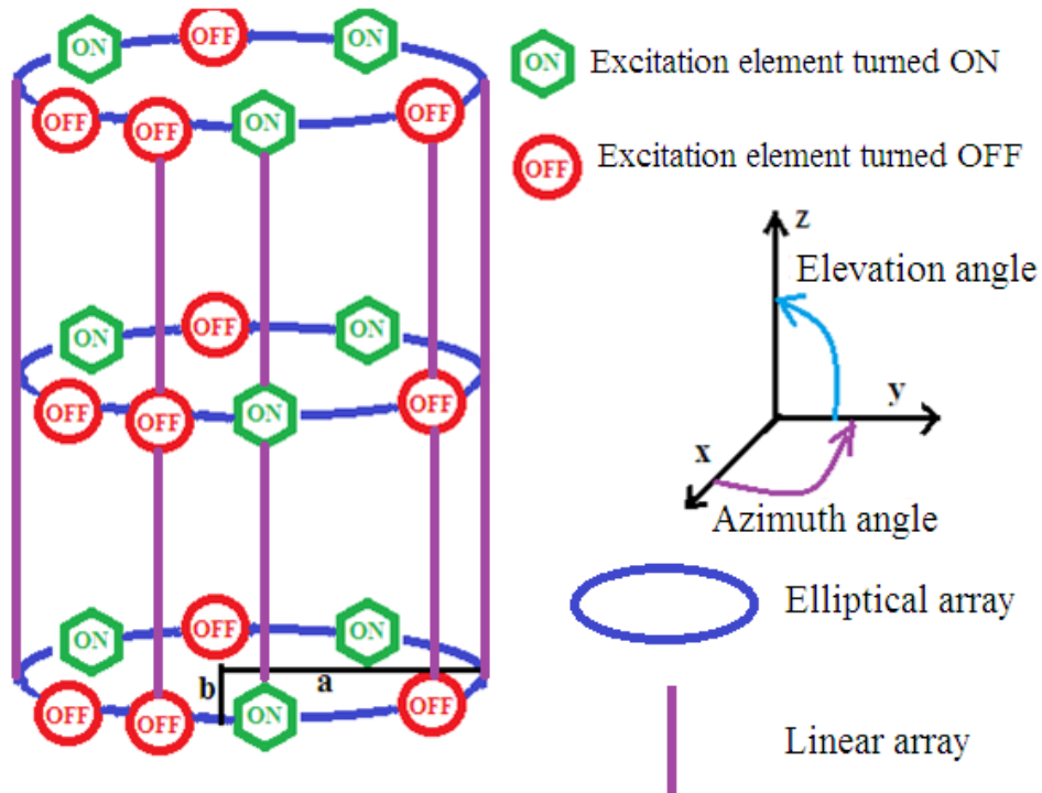
Figure 2. Proposed antenna array geometrical configuration and position of the array elements.
