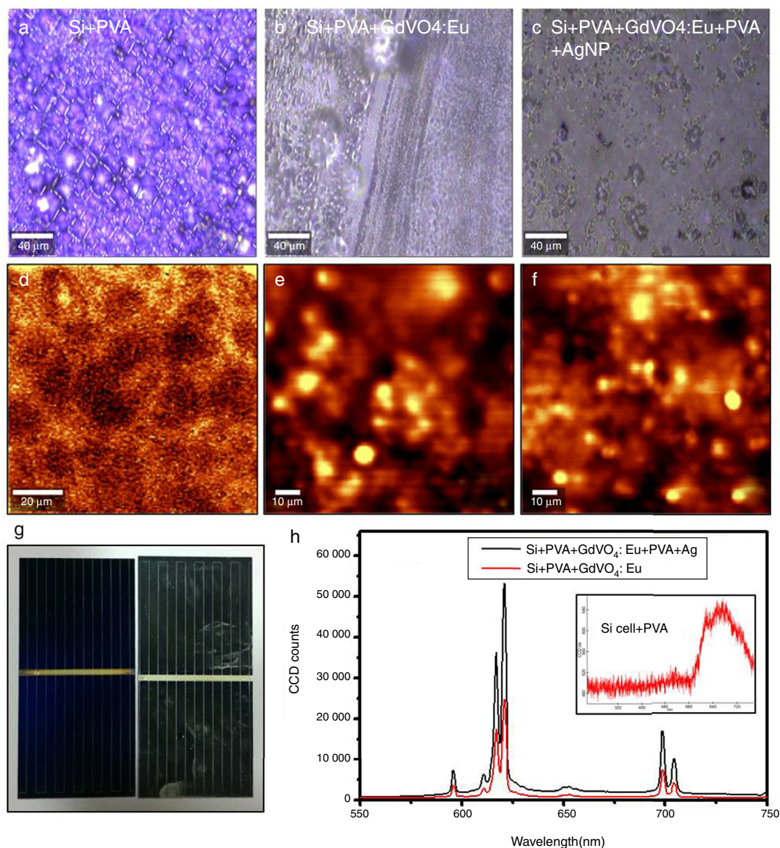
Fig. 6. Optical images and confocal fluorescence map of: (a) and (d), the Si Cell+PVA; (b) and (e), the Si cell+PVA+GdVO 4 :Eu; (c) and (f), the Si cell +PVA +GdVO 4 :Eu +PVA + Ag NP; (g), digital image of the bare Si cell (left) PVA +GdVO 4 :Eu +PVA + Ag NP deposited on the Si cell; (h) corresponding spectra comparing the Eu 3+ emission intensity with and without Ag NPs suggesting enhancement of fluorescence, the inset shows the emission from the Si cell with the PVA layer under the same experimental conditions.
