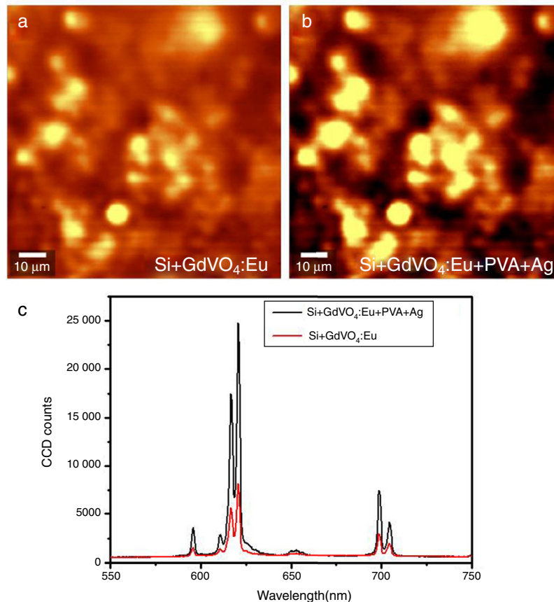
Fig. 4. Confocal fluorescence map of (a) GdVO 4 :Eu; (b) GdVO 4 :Eu + PVA + Ag NP deposited on the Si cell; (c) corresponding spectra comparing the Eu 3+ emission intensity with and without Ag NPs suggesting enhancement of fluorescence.
